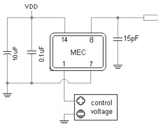
[ Thru - Hole Type ] CMOS Square Wave Test Circuit
