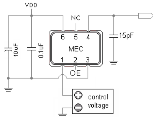
[ SMD 6 pads ] CMOS Square Wave Test Circuit
